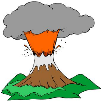
volcano
