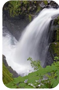
waterfall
