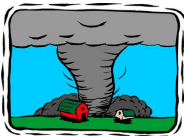
tornado
